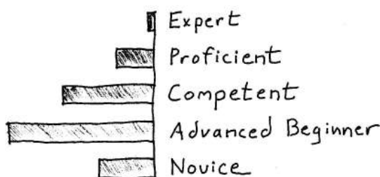
Figure 2.4: Skill distribution
